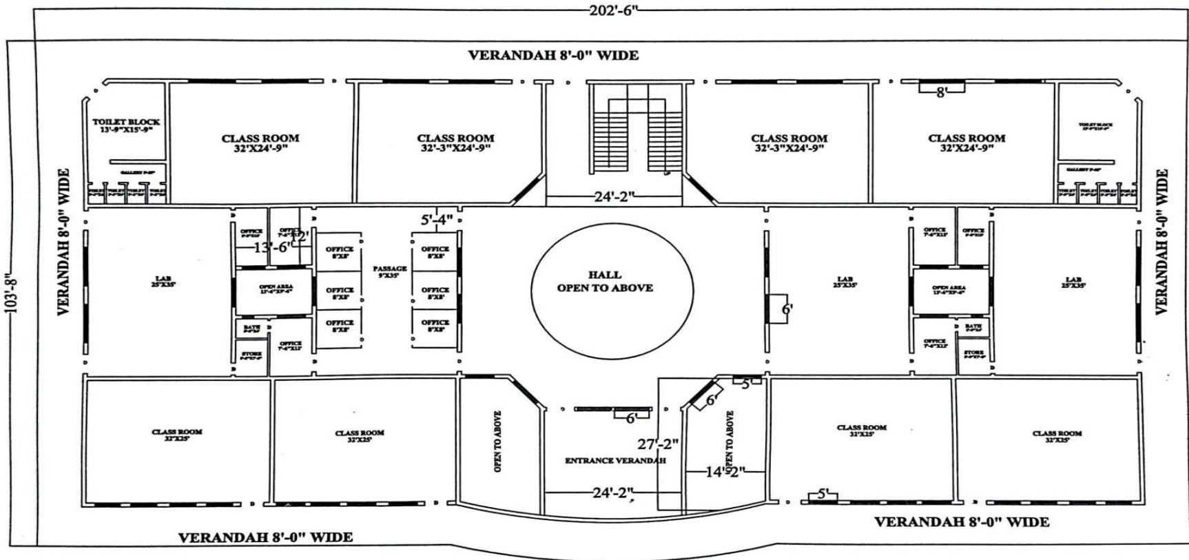
GROUND FLOOR PLAN B.S BLOCK EXISTING
