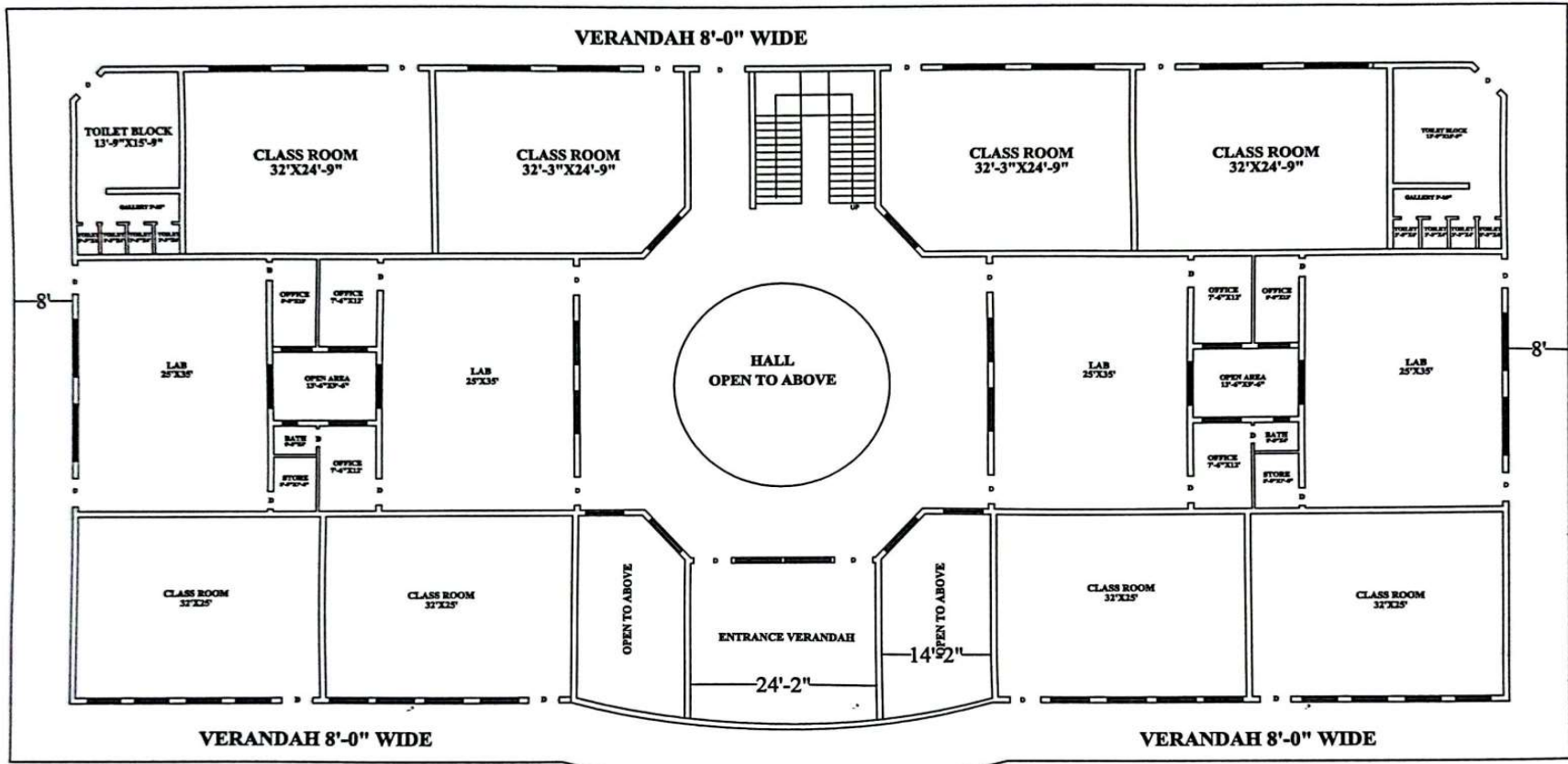
FIRST FLOOR PLAN B.S BLOCK EXISTING
